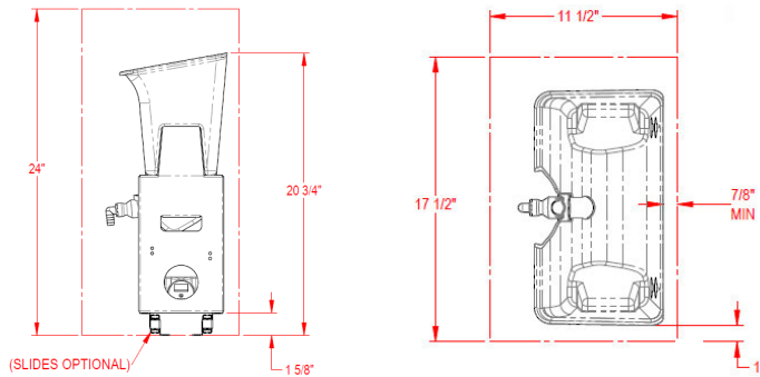
CDS-1E Electric Dispensing System
