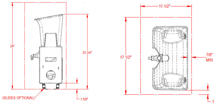
CDS-1G Gas Operated Dispensing System
