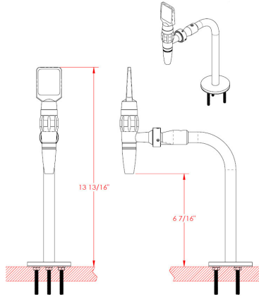
WB-RT-1 Single Round Tower
