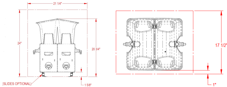
CDS-2E Dual Electric Dispensing System
