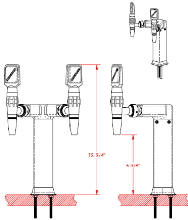
WB-ST-2 Dual Square Tower
